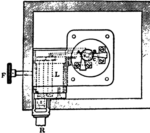
FIG. 57.—The Manograph.
